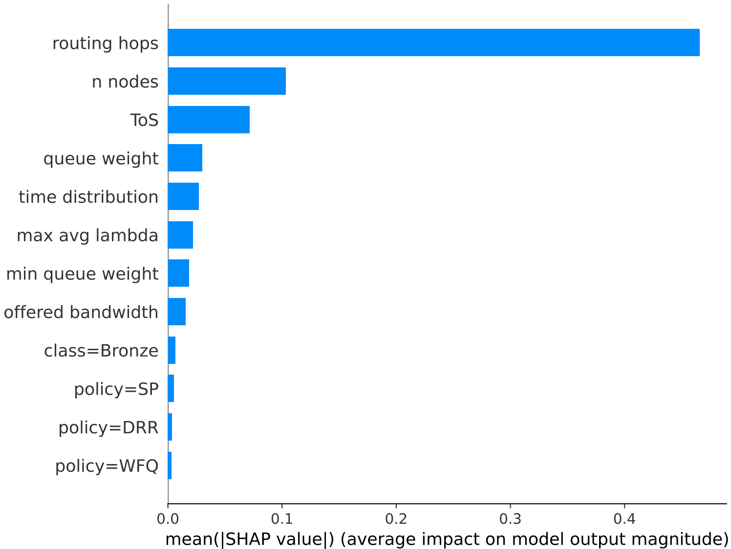
Global feature importance (mean |SHAP|)
